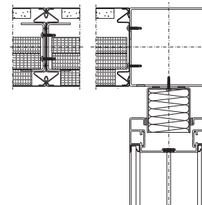
slim ceiling
