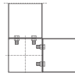
without ceiling
